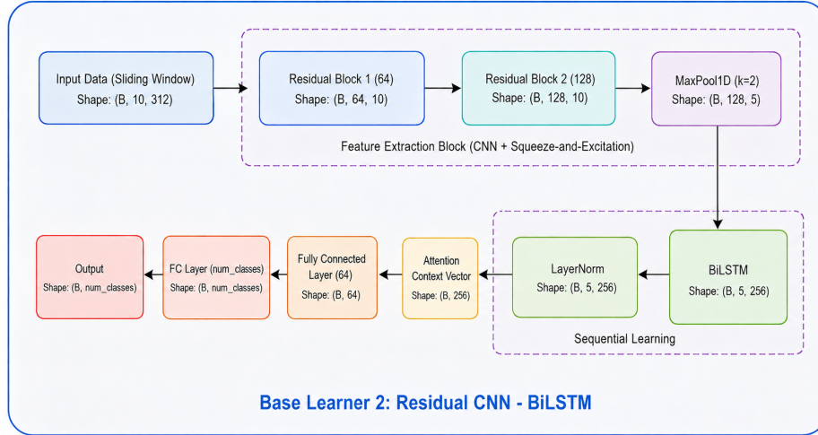
Figure 3.3: Temporal base learner based on residual CNN blocks and BiLSTM attention.
