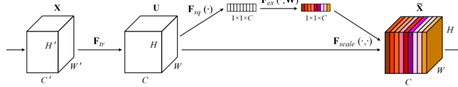
Figure 2.3: Squeeze-and-Excitation block.
