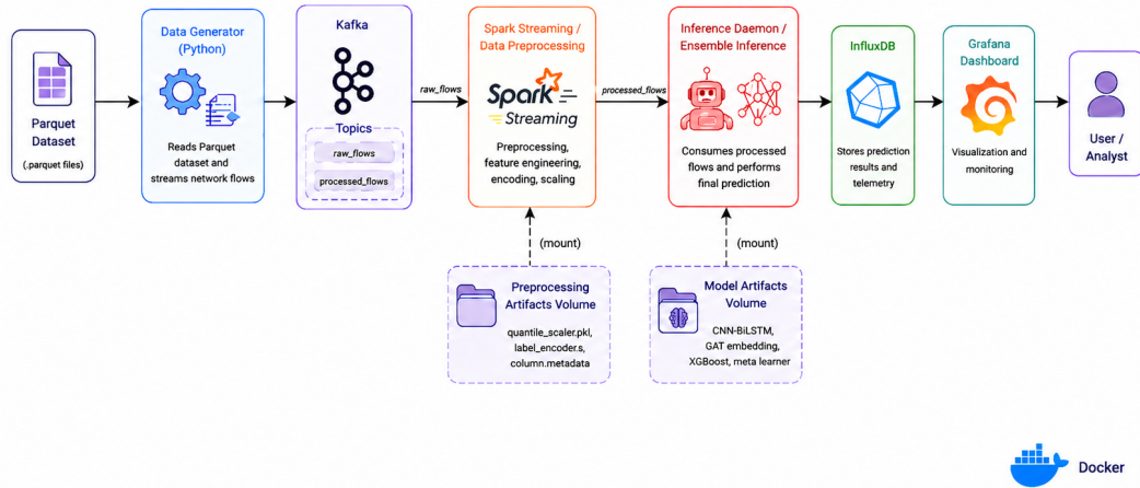
Figure 7.1: Deployment diagram of the proposed ensemble architecture.
